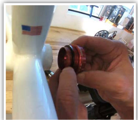
6. Insert non-drive side cup into frame, add supplied spacers as necessary to achieve proper bottom bracket width.
