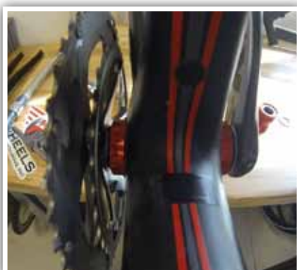
11. Add spacers as necessary to take up any play, remove spacers as necessary if binding occurs.
